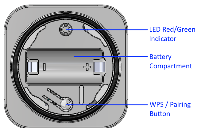
Smart Water Sensor (top view open) —
